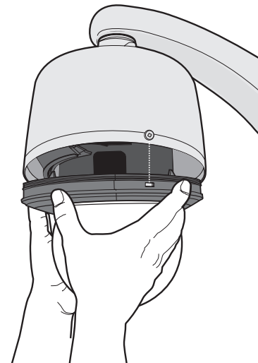
Figure 2. Installing the Lower Dome (Pendant Model Shown)
